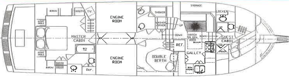
56 Cockpit Plan A
