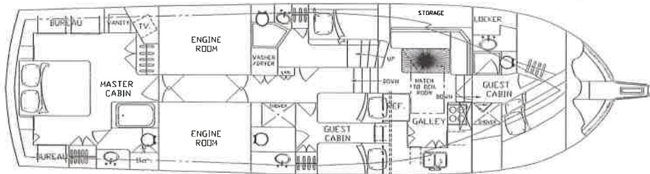
56 Cabin Deck Plan A
