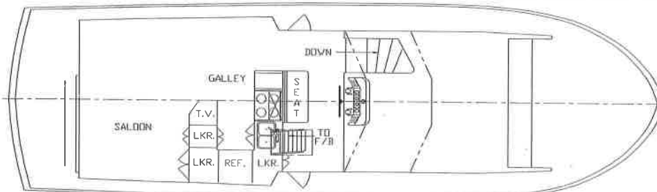
52 EDH Saloon Deck Plan, Galley Up
