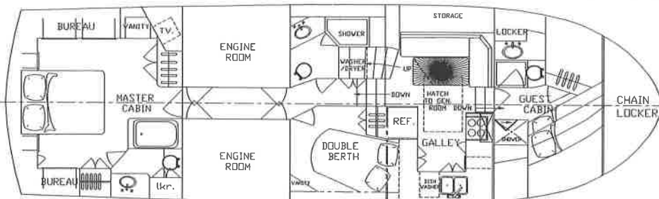
52 Cabin Deck Plan A
