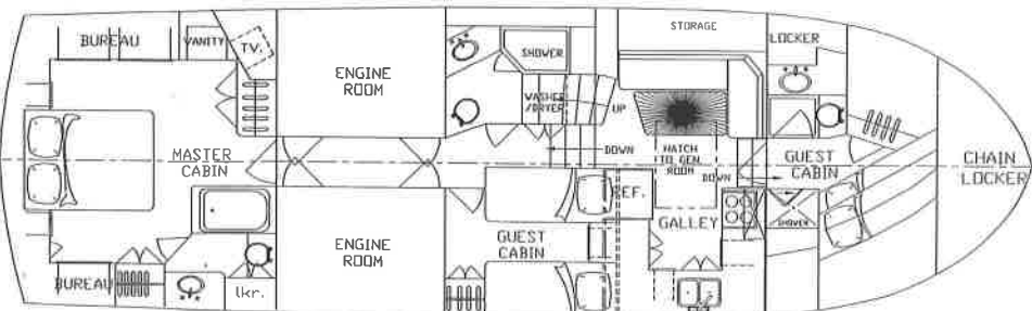
52 Cabin Deck Plan B
