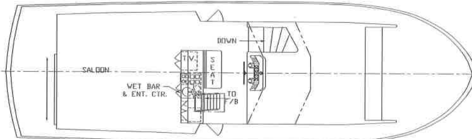
52 Extended Deckhouse Saloon Deck Plan
